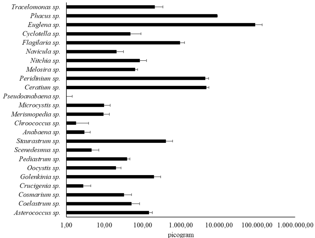
Figure 4 Carbon content in each genus of phytoplankton in Jatigede Reservoir
