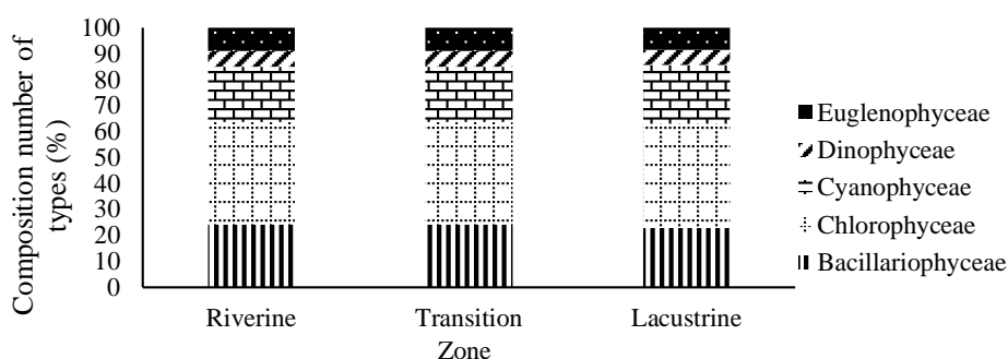
Figure 2 Composition of the number of types of phytoplankton in Jatigede Reservoir
