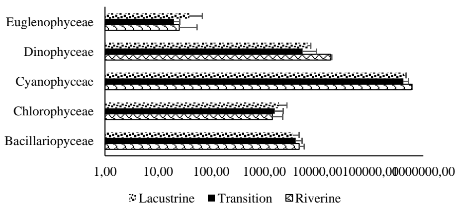
Figure 3 Phytoplankton abundance in Jatigede Reservoir
