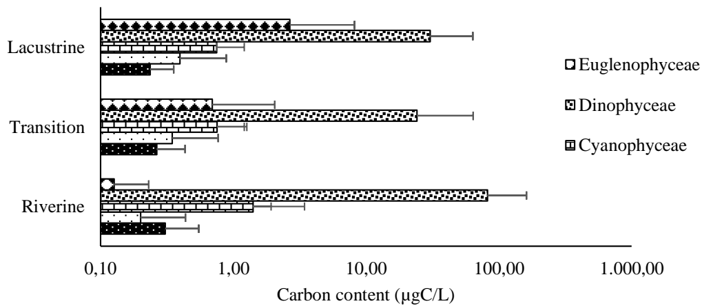
Figure 5 Carbon content in each class of phytoplankton in Jatigede Reservoir
